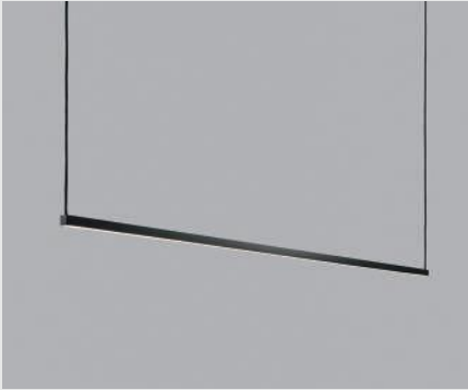
STRIPE S2000 / Black / ART. No 27071 Design: Ronni Gol 1x33W LED - 230V - IP20 indoor only CRI > 90 - 2700K - Dimmable Dimensions: 2000 x 15 mm
